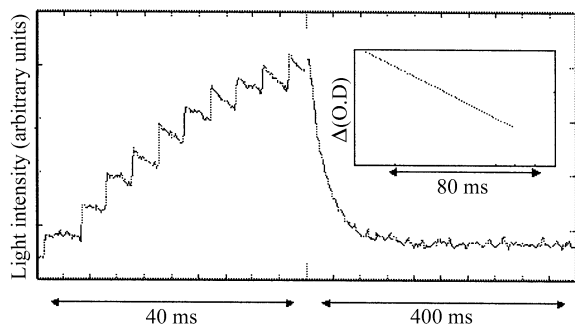
Fig. 1 Computer output of light intensity vs. time. Formation and decomposition of [\text{LCu}^{\text{II}}\text{-CH}_3\text{CO}_2]^{+} complex. Solution composition: 2 \times 10^{-3} M L, 1 \times 10^{-3} M \text{Cu}^{+}_{\text{aq}} and 0.1 M Acetate, \text{N}_2\text{O} saturation, pH 7.5. 10 pulses delivered, pressure = 1500 bar. Inset: kinetics of the disappearance of the \text{LCu}^{\text{II}}\text{-CHCO}_2^{-} complex, fit to a single exponential.
