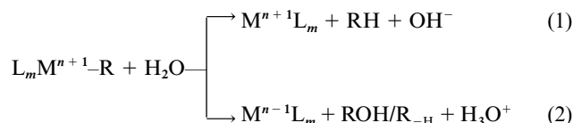
Scheme 1 General base catalysis of heterolysis of \text{Cr}^{\text{III}}\text{--C} bonds in [(\text{H}_2\text{O})_5\text{Cr}^{\text{III}}\text{--R}]^{2+} .
